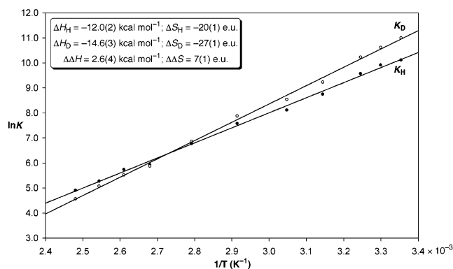
Figure 7. van't Hoff plot for oxidative addition of H 2 and D 2 to Ir(PMe 2 Ph) 2 (CO)Cl in benzene over the range 25–130 °C.
