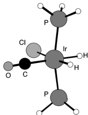
Figure 2. Geometry optimized structure of Ir(PH 3 ) 2 (CO)ClH 2 . Selected bond lengths (Å): Ir–P 2.317 and 2.318, Ir–H( trans to Cl) 1.588, Ir–H( trans to CO) 1.632, Ir–Cl 2.529, Ir–CO 1.951.
