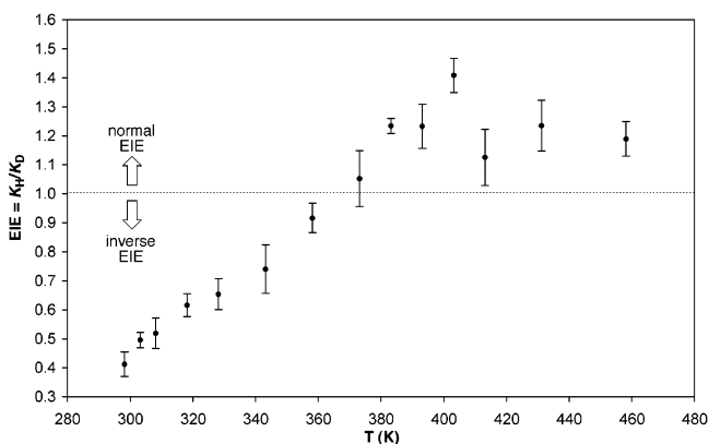
Figure 6. Temperature dependence of the EIE for oxidative addition of H 2 and D 2 to Ir(PMe 2 Ph) 2 (CO)Cl in benzene.
