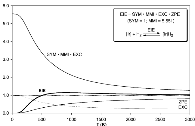
Figure 3. Calculated EIE as a function of temperature for oxidative addition of H 2 and D 2 to Ir(PH 3 ) 2 (CO)Cl expressed in terms of SYM, MMI, EXC, and ZPE components.
