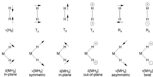
Figure 1. Vibrational modes associated with a C 2 -symmetric [MH 2 ] fragment and the vibrational, translational, and rotational modes of H 2 from which they are derived.
