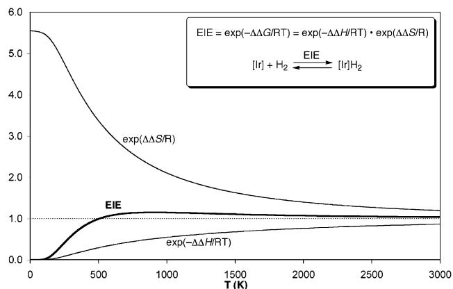
Figure 4. Calculated EIE as a function of temperature for oxidative addition of H 2 and D 2 to Ir(PH 3 ) 2 (CO)Cl, expressed in terms of \exp(-\Delta\Delta H/RT) and \exp(\Delta\Delta S/R) .
