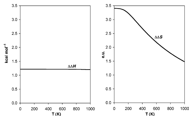
Figure 5. Calculated temperature dependence of \Delta\Delta H = \Delta H_{\text{H}} - \Delta H_{\text{D}} and \Delta\Delta S = \Delta S_{\text{H}} - \Delta S_{\text{D}} . \Delta\Delta H varies from 1.22 to 1.20 kcal mol -1 from 0 to 1000 K, whereas \Delta\Delta S varies from 3.41 to 1.48 e.u.
